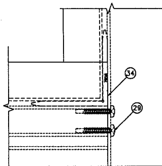
SASH CORNER ASSEMBLY - SQ. CUT, END COPED, CORNER KEYED, AND MECH. FASTENED.
