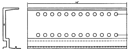
■SUBHEAD STIFFENER
